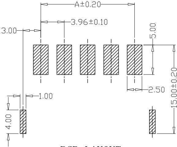
PCB LAYOUT
